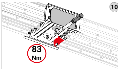
10- Adjust the torque wrench to 83 Nm (60 lbft) and tighten the joint nut.
