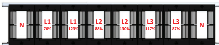
Non-Optimized Conductor Arrangement (Load current unbalanced)
